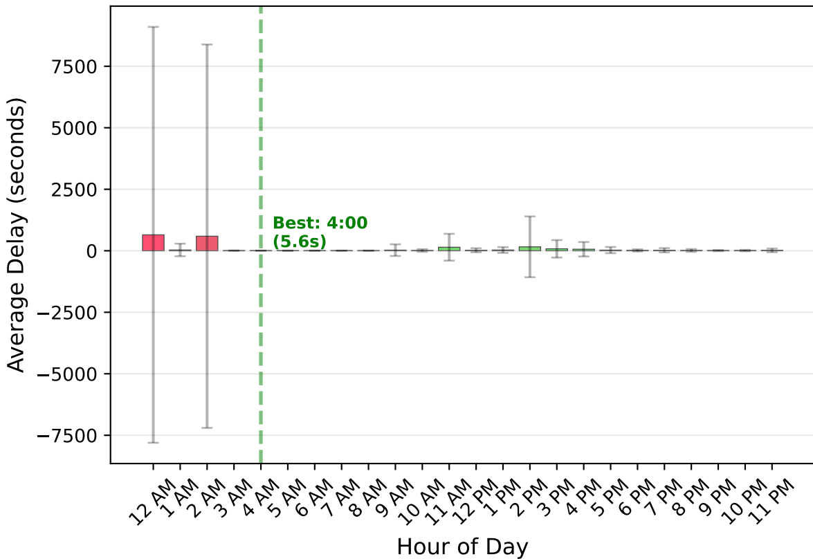
Average Queuing Delay by Hour of Day - 4 Cores
